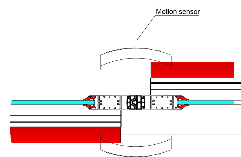
DETAIL C
