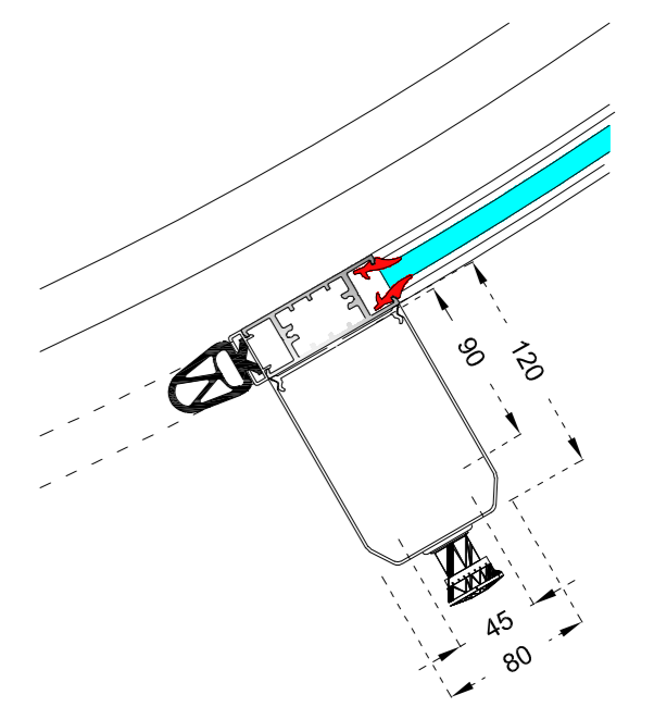
DETAIL A
