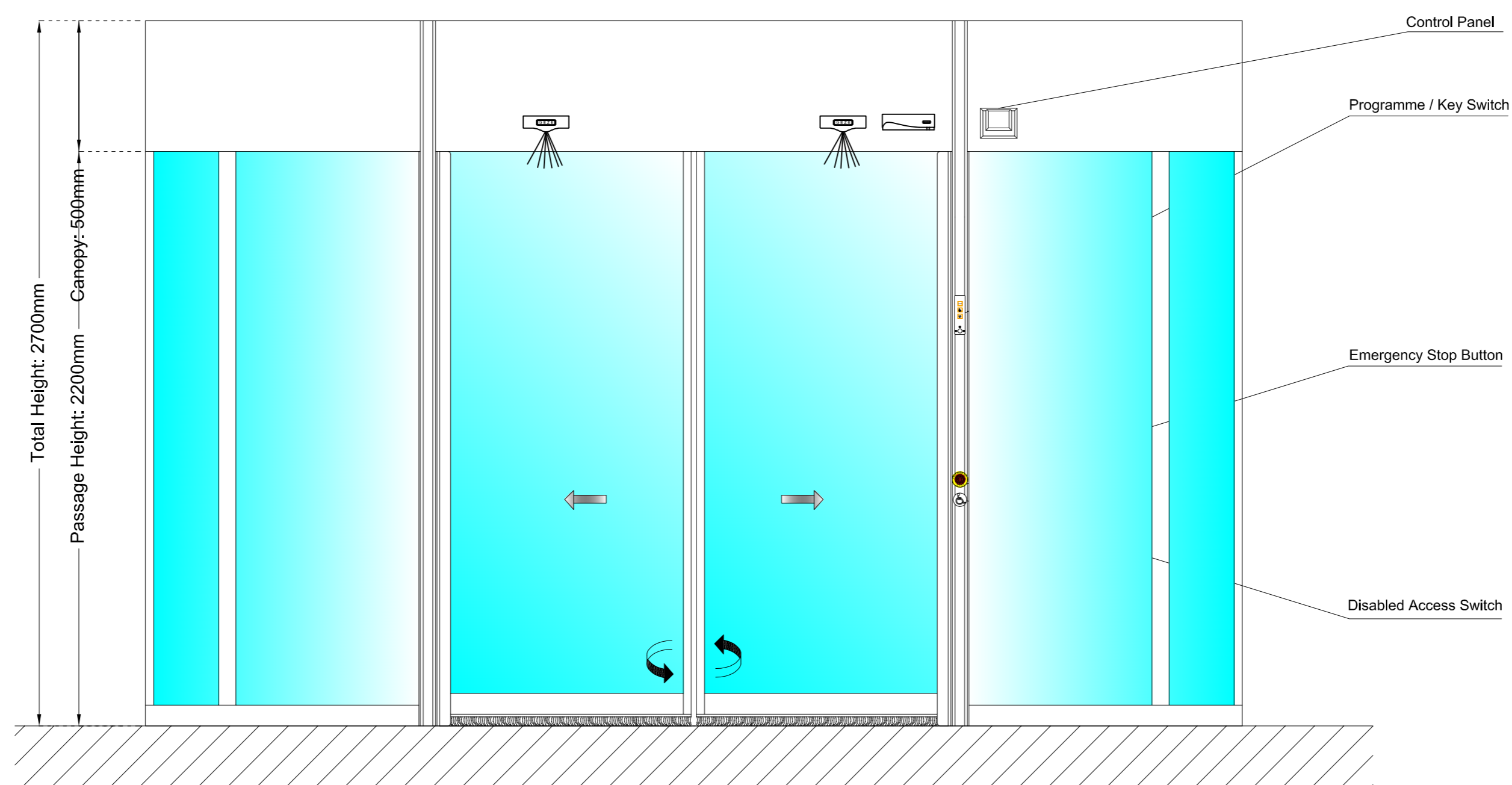
FRONT VIEW
